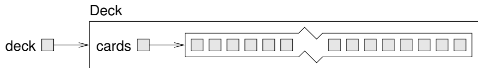
Figure 13.1: Memory diagram of an unpopulated Deck object.
