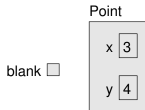
Figure 10.7: Memory diagram showing the effect of setting a variable to null .
