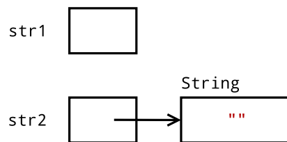
Figure 9.5: Memory diagram of null and empty string.
